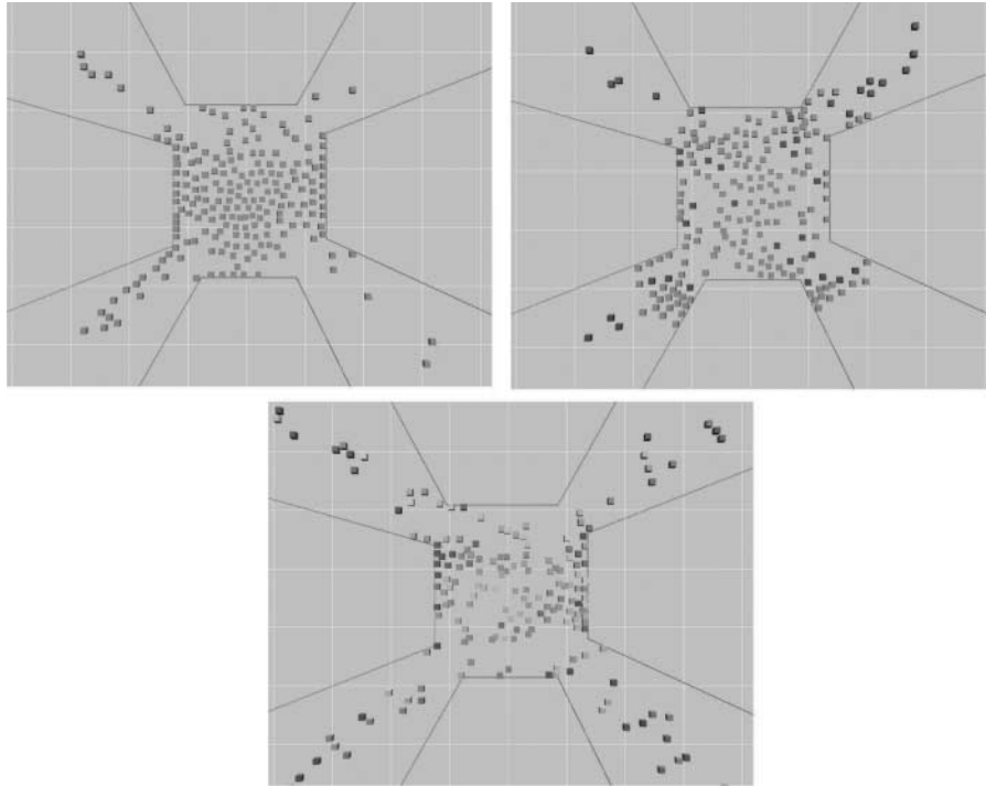
FIGURE 10. Agent diversity and complexity of crowd behavior can be adjusted with our model (left to right: uniform, 80% calm 20% aggressive, diverse agents).
