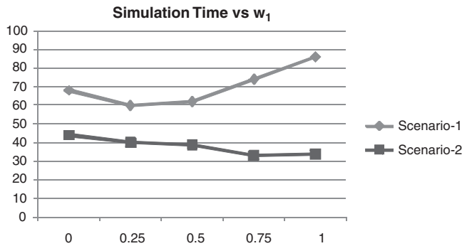
FIGURE 6. Simulation times of two scenarios under different w_1 assignments; w_1 determines the contribution of the entropy map in behavior map construction.
