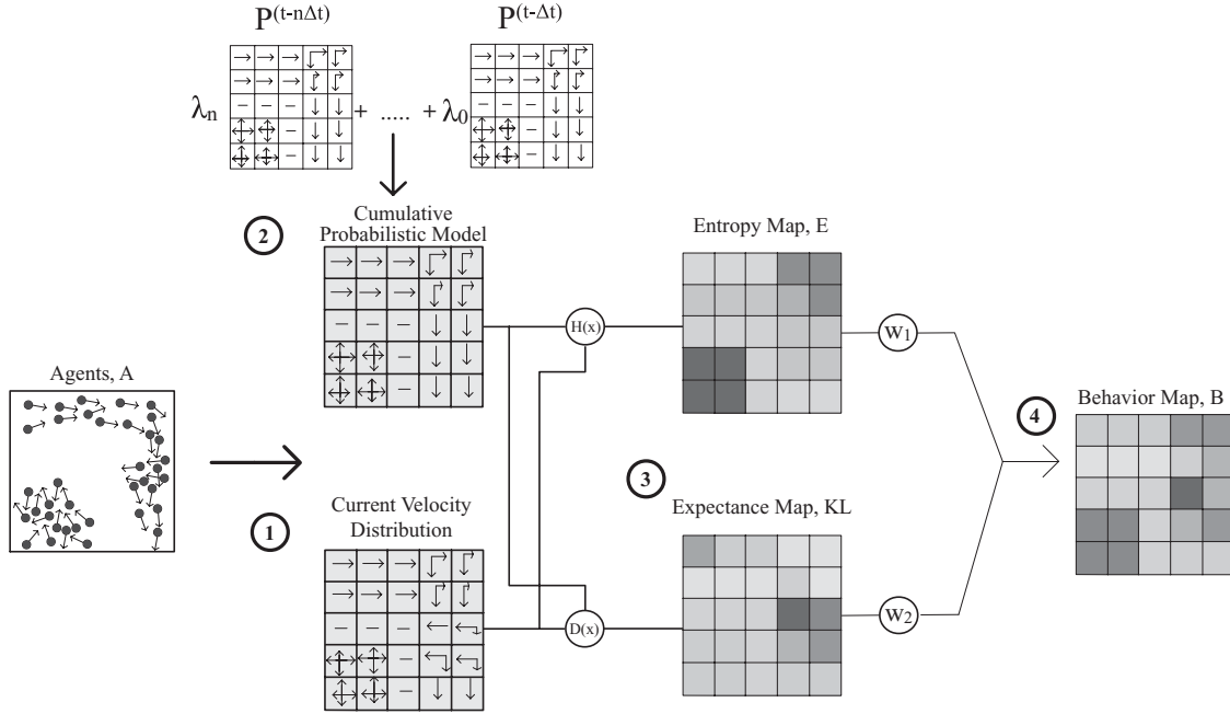
FIGURE 2. Behavior map construction. (1) Current distribution of crowd locomotion. (2) Older distributions are merged with a temporal filter. (3) Entropy and expectance maps are calculated. (4) Behavior map is constructed with convex combination using user-defined weights.
