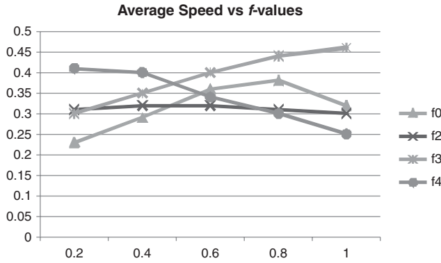
FIGURE 5. Average speed of agents over varying f values.
