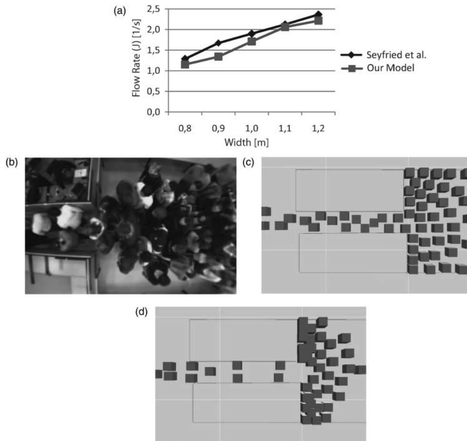
FIGURE 9. (a) Flow vs. width of exit. (b) Real-world scenario. (c) Our test environment with less aggressive agents. (d) Clogging occurs when agents are more aggressive.
