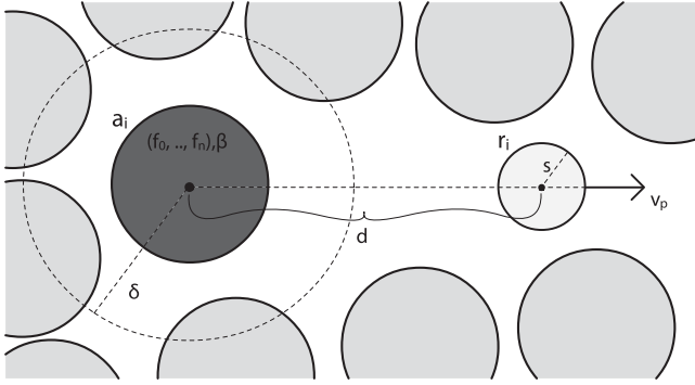
FIGURE 3. A composite agent a_i , its associated proxy agent r_i and certain features of agent representation.
