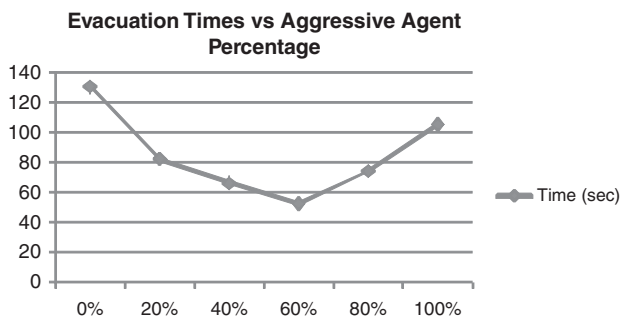
FIGURE 7. Simulation times of the evacuation scenario with different aggressive agent percentages.
