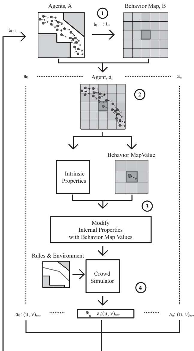
FIGURE 1. Overall structure of our model. (1) Behavior map is produced. (2) Agents are assigned a specific cell value. (3) Agents' intrinsic properties are modified with behavior map value. (4) Agents' locomotion is determined by simulator.
