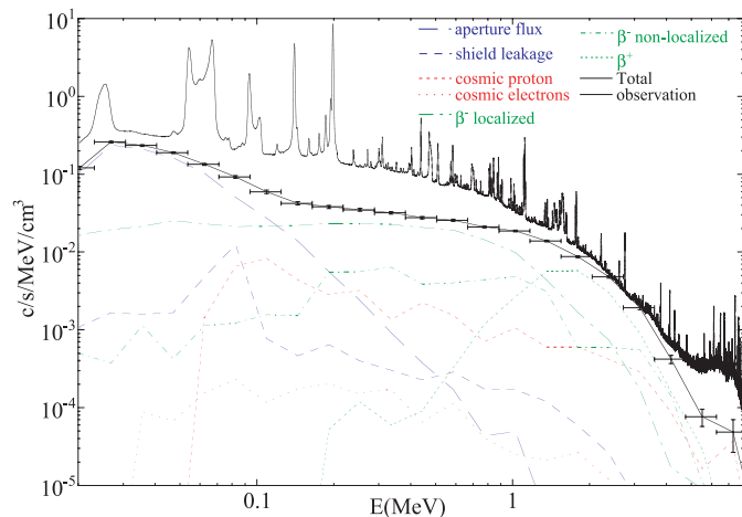
Fig. 10. Comparison of continuum background spectrum estimated by simulation before the launch of INTEGRAL with the measurements. Background components are shown separately.
