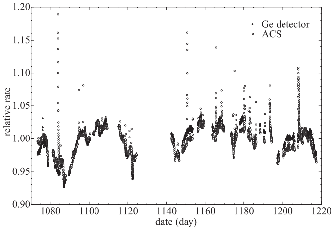
Fig. 6. Variation of the total GeD and ACS rates as a function of time. The large excesses in the ACS rate are due solar flares and electron belts entry. Dates are relative to 2000 January 01, 0h00.
