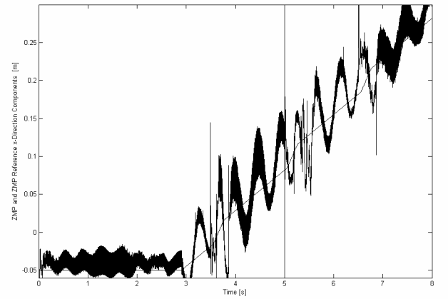
Fig. 14. ZMP and ZMP reference x-direction components
