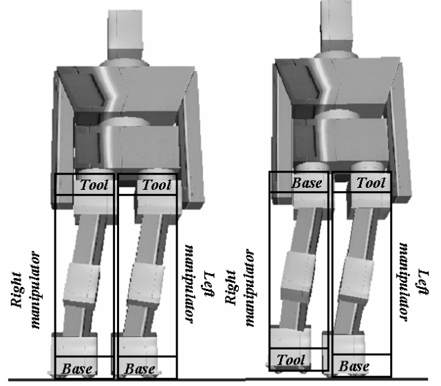
Fig. 10. The robot in the double support phase can be regarded as a trunk manipulated by two six-DOF manipulators based on the ground (left). The robot in swing phases can be seen as a ground based manipulator and a second manipulator based at the hip (right).
