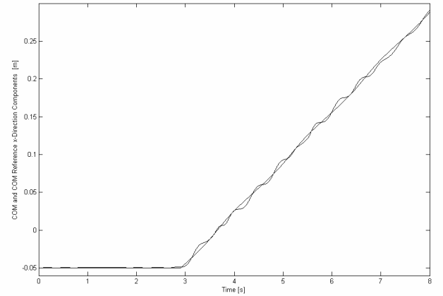
Fig. 13. CoM and CoM reference x-direction components
