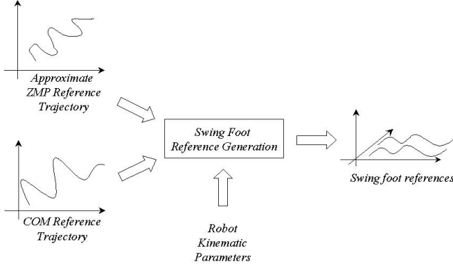
Fig. 8. The swing foot references are obtained from ZMP and CoM references.
